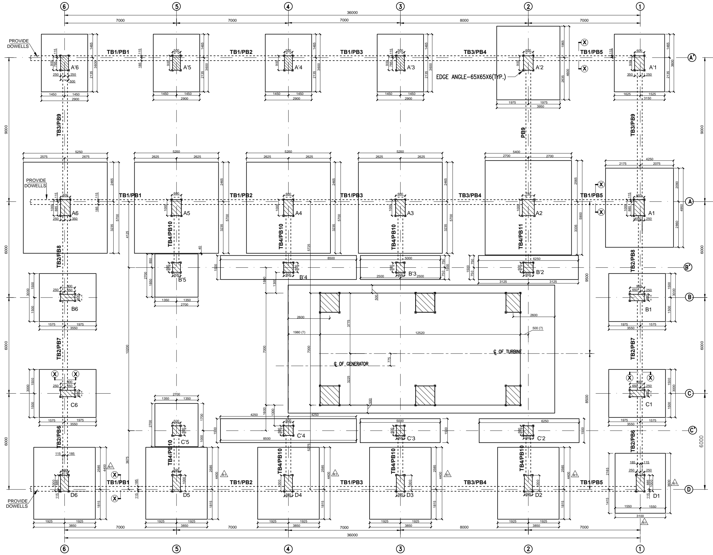
FOUNDATION PLAN
