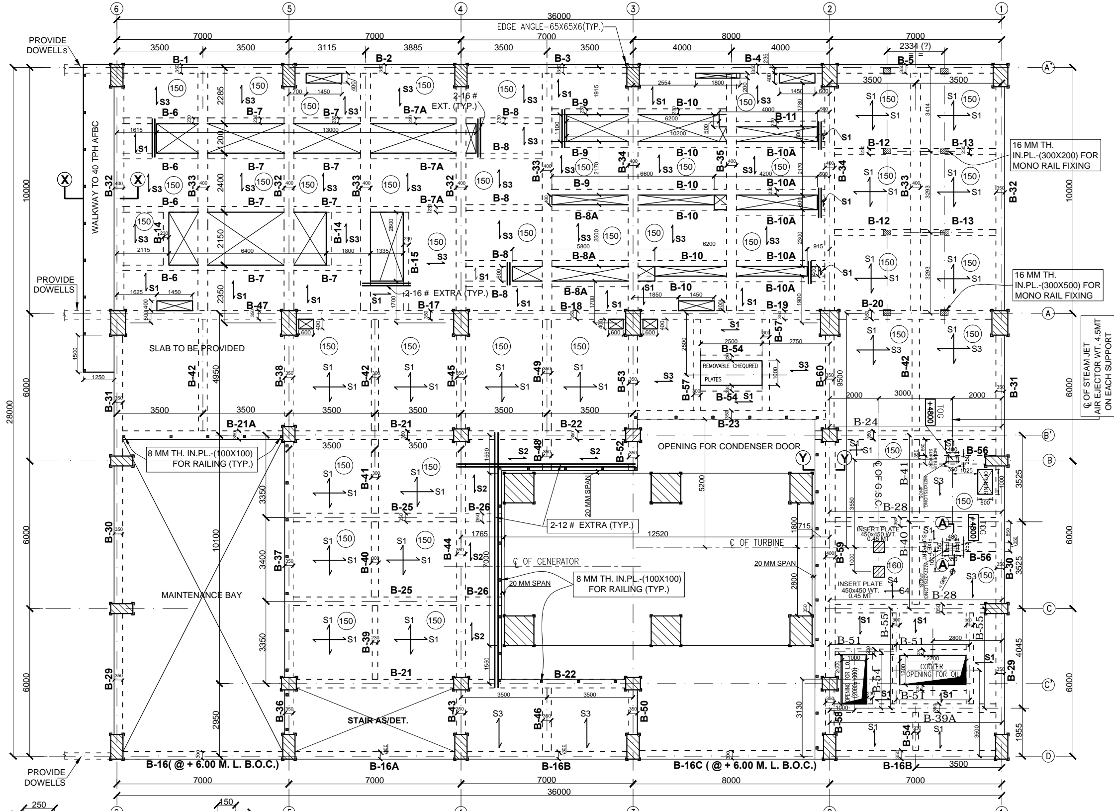
PLAN SHOWING BEAMS & SLABS DET. @+ 4.50M. LVL. (T.O.C.) OF T. G. BUILDING
