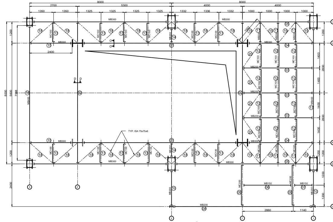
FLOOR DETAIL +9550 02
