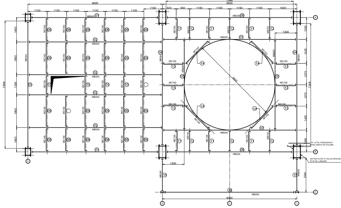
FLOOR DETAIL +16310
