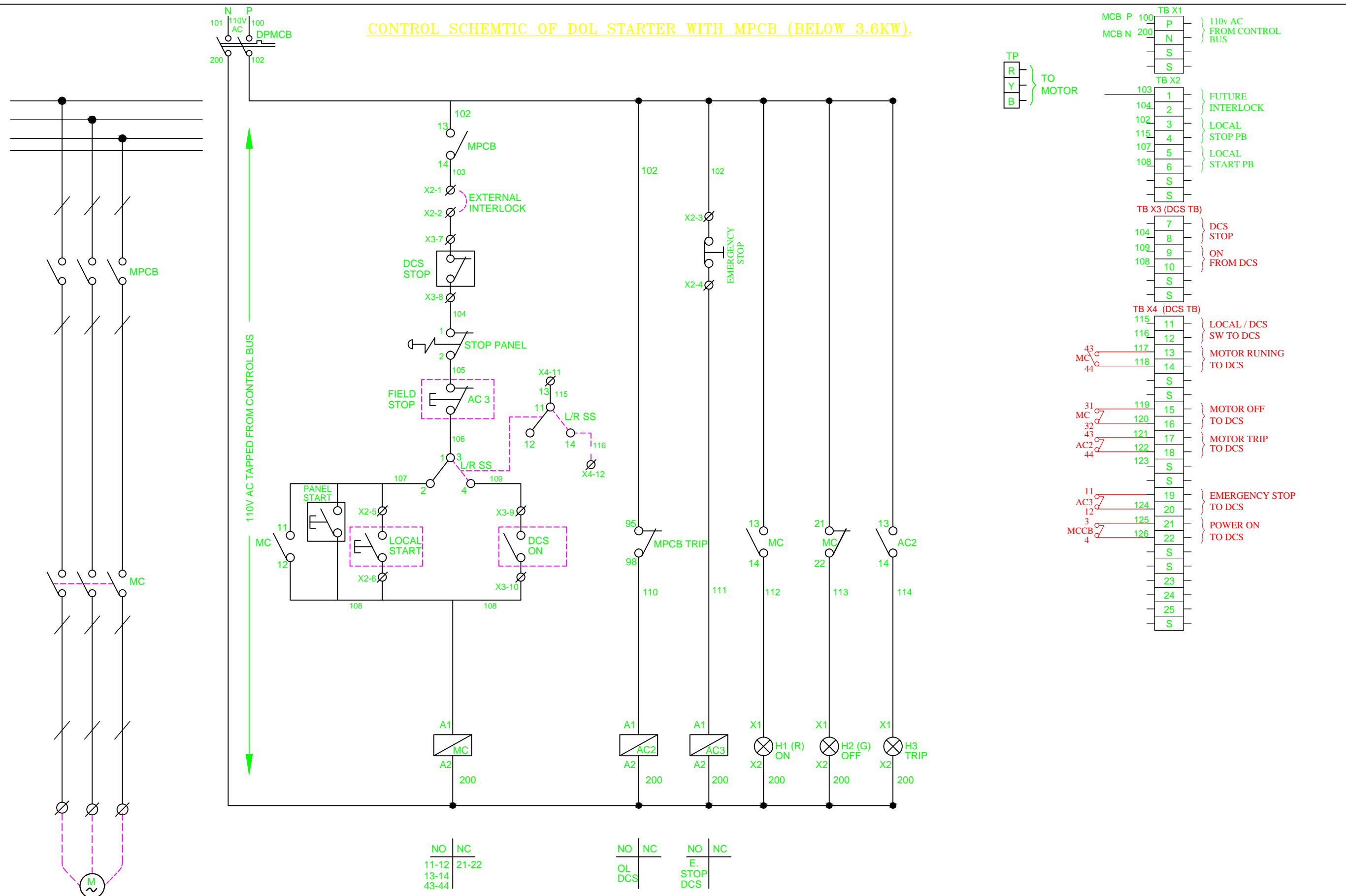
WIRING DIAGRAM OF DOL FEEDER (SCHEME :-2)
